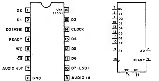
SN76489AN (TI) IIL PROGRAMMABLE SOUND GENERATION CONTROLLER — TOP VIEW —
